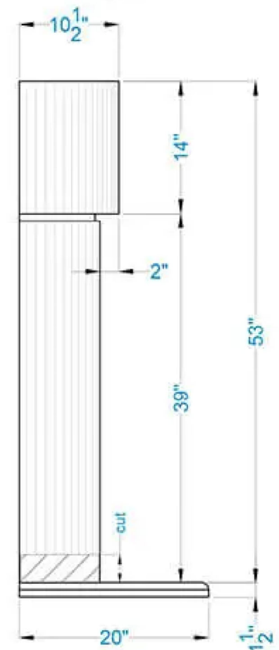
SIDE VIEW
