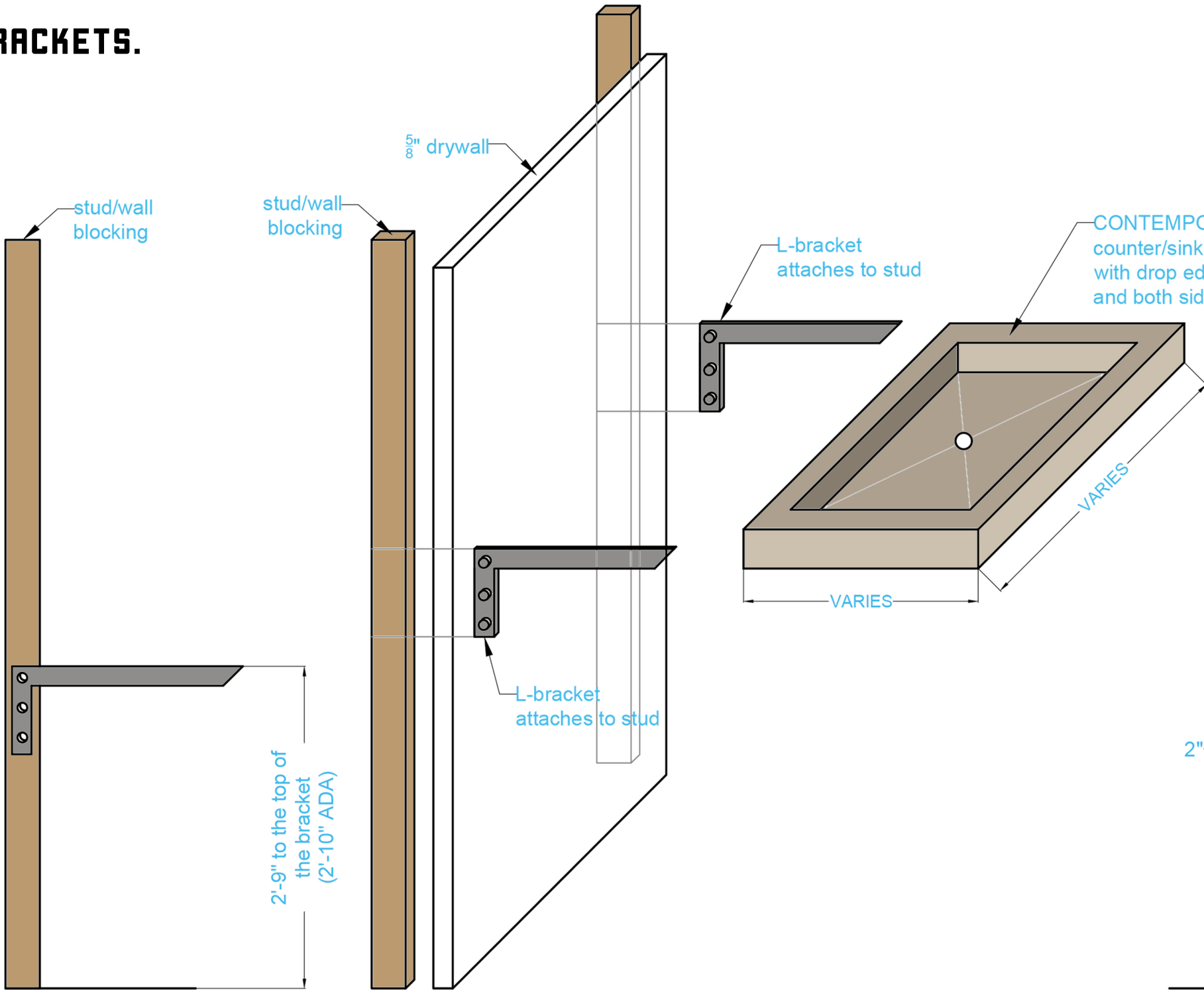
Side view showing recommended height to install T-brackets
