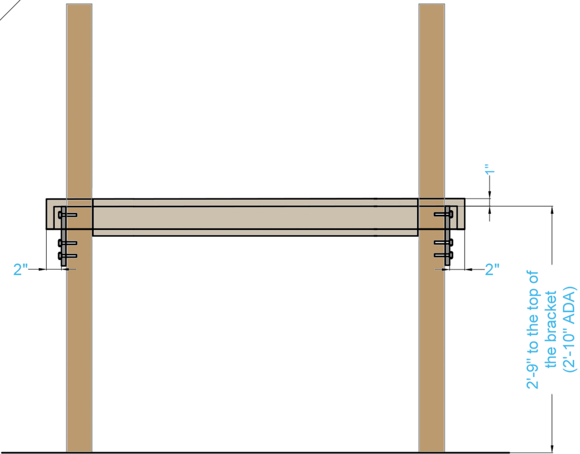
Back view showing placement of T-brackets
