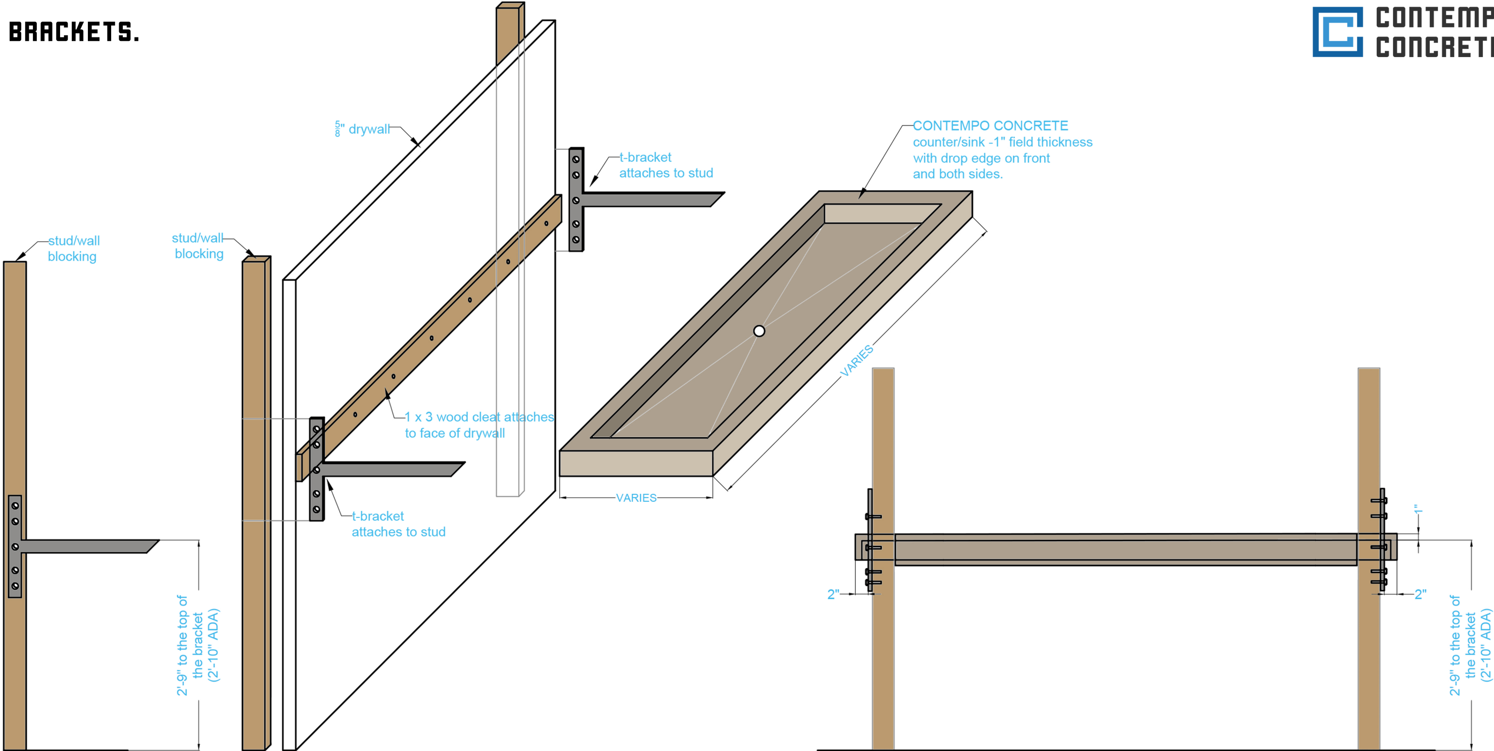
Back view showing placement of T-brackets
