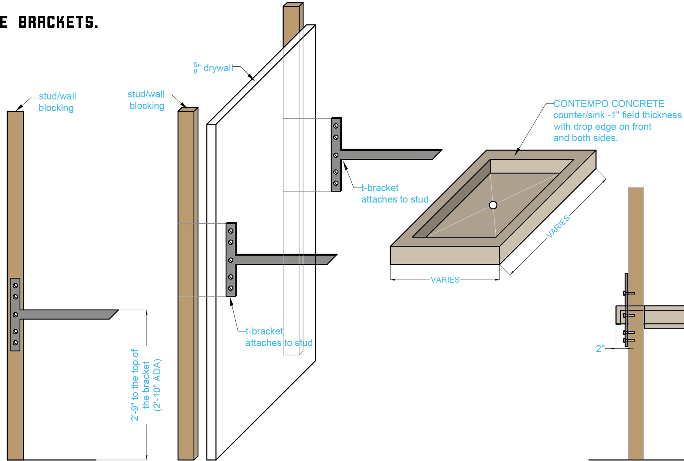
Back view showing placement of T-brackets
