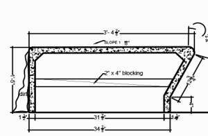
SECTION B-B1
