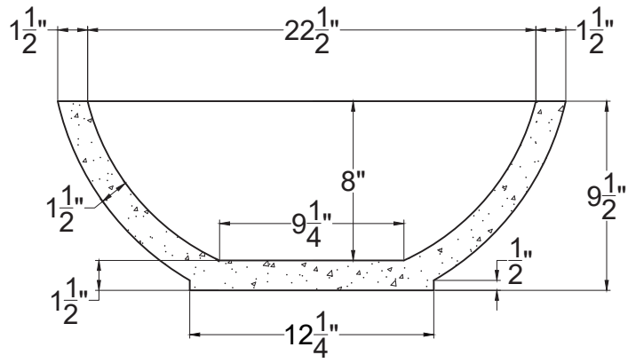
SECTION A
