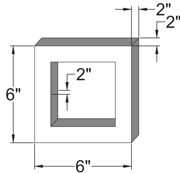
AXONOMETRIC VIEW
