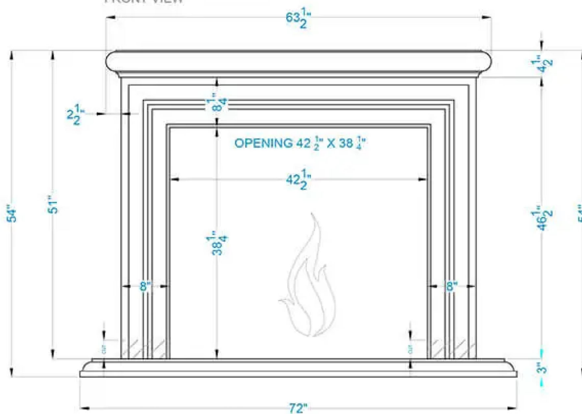
FRONT VIEW
