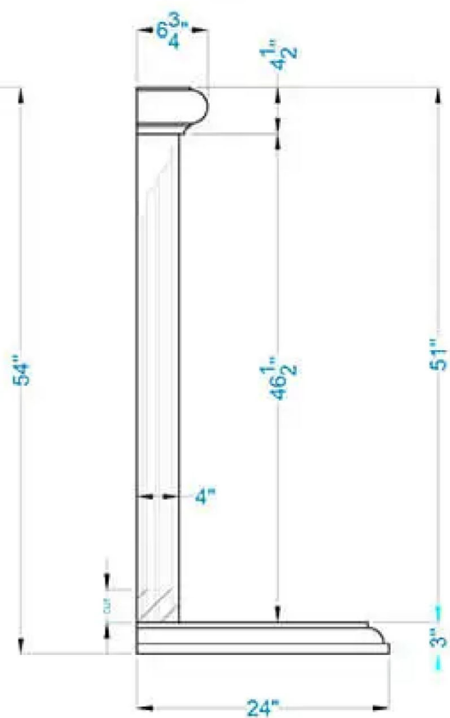
SIDE VIEW
