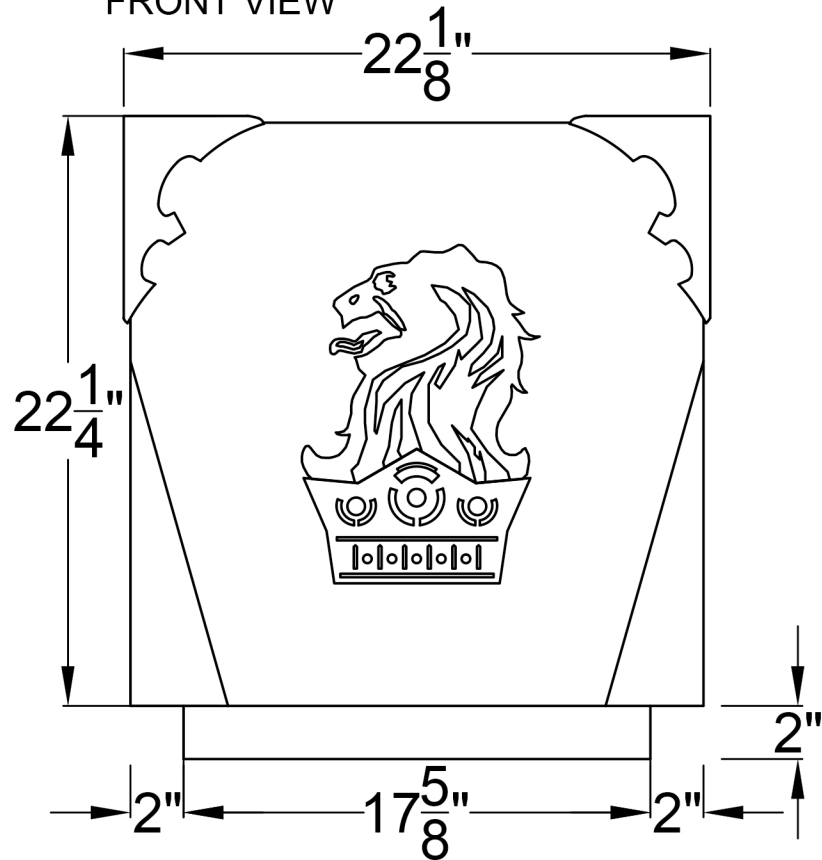
FRONT VIEW
