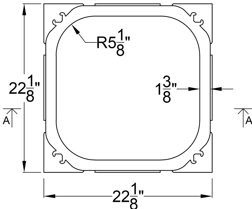
TOP VIEW
